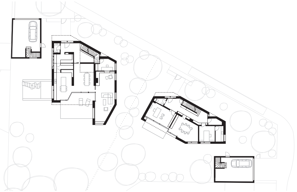
erdgeschoss . ground floor
